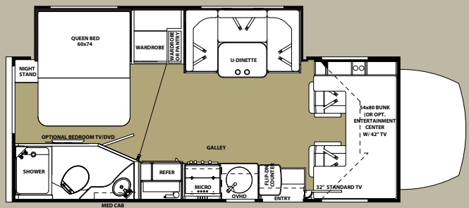
MBS 2401W
